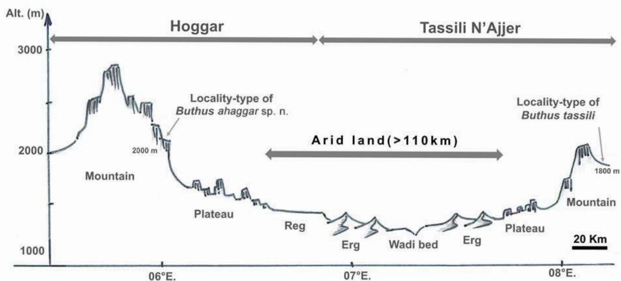
Fig. 29. Schematic relief showing the ecological gradients between the Hoggar and Tassili N'Ajjer Massifs.
